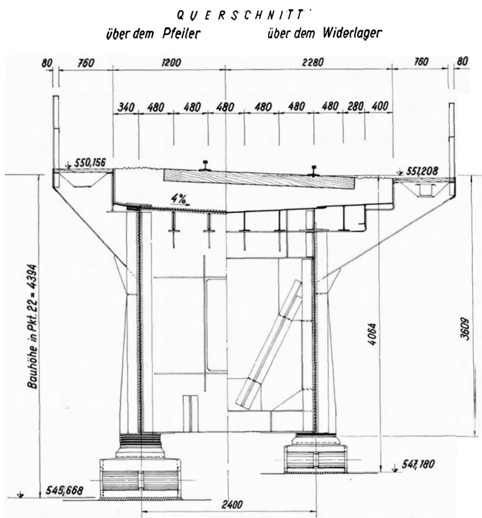
Fig. 4a: Cross-Section
