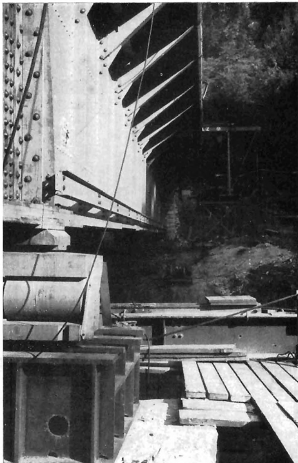
Fig. 4e: Bearings and girder grating on the pier
